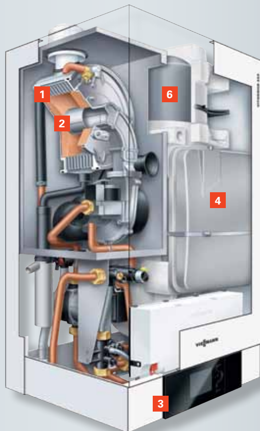
Vitodens 222-W
